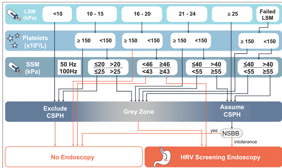
Figure 3 Example of an integration algorithm based on LSM by TE, platelets and SSM by TE for detection of CSPH and screening for HRV in patients with cACLD. Flowchart based on the following algorithms: Baveno VI criteria [25], combined Baveno VI + SSM algorithm by Colecchia et al [57] and Vanderschueren et al [58], Baveno VII criteria [25], Baveno VII + SSM criteria by Dajti et al [16,43] and Jachs et al [16]. LSM, liver stiffness measurement; TE, transient elastography; SSM, spleen stiffness measurement; CSPH, clinically significant portal hypertension; NSBB, non-selective beta-blocker; CI, contra-indication; HRV, high-risk varices; cACLD, compensated advanced chronic liver disease; TE, transient elastography
