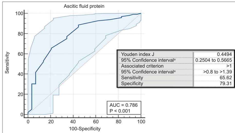
Figure 2 Area under the receiver operating characteristic curve (AUROC) to predict accuracy of ascitic fluid protein for left ventricular diastolic dysfunction (LVDD)
