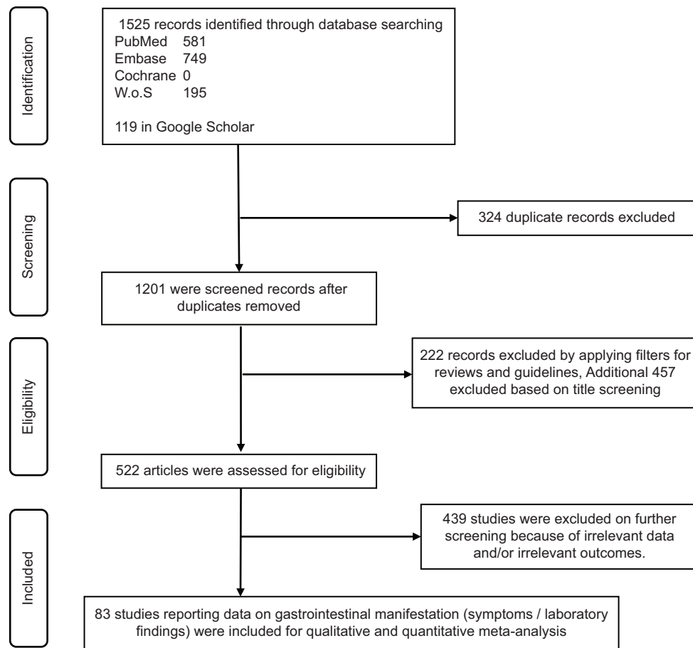
Figure 1 PRISMA diagram
